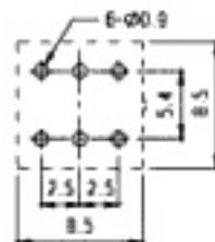
PCB LAYOUT
