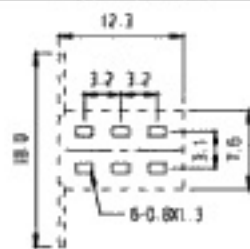
PCB LAYOUT
