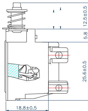
SCHEMATIC DIAGRAM
