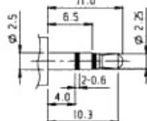
MATING PLUG
